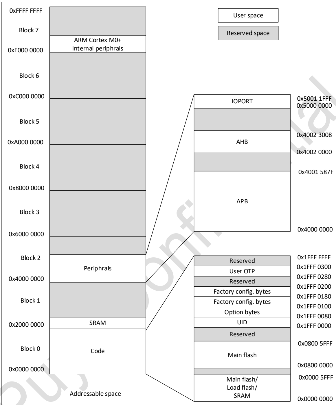
Figure 4-1 Memory mapping
